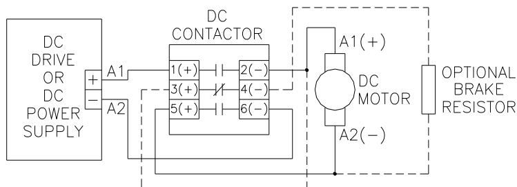
Typical DC Motor and Drive Application
